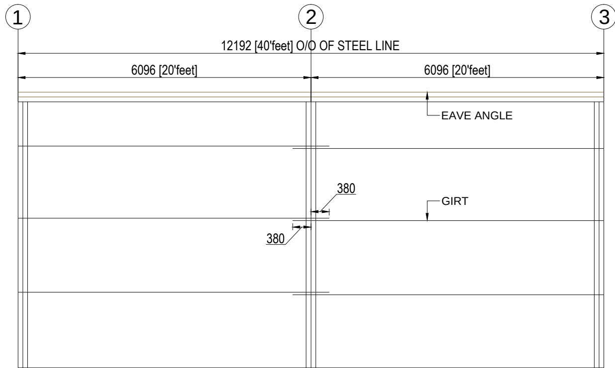
SIDE WALL FRAMING @ GRID-C
