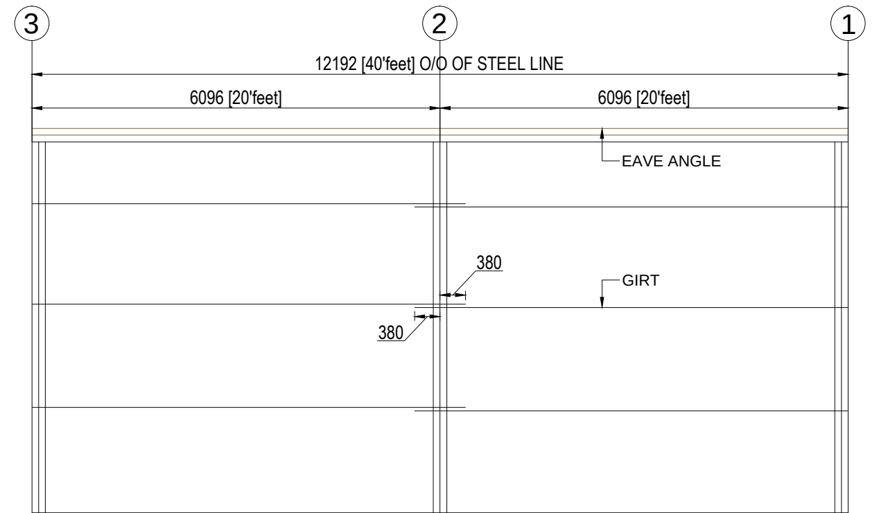
SIDE WALL FRAMING @ GRID-A
