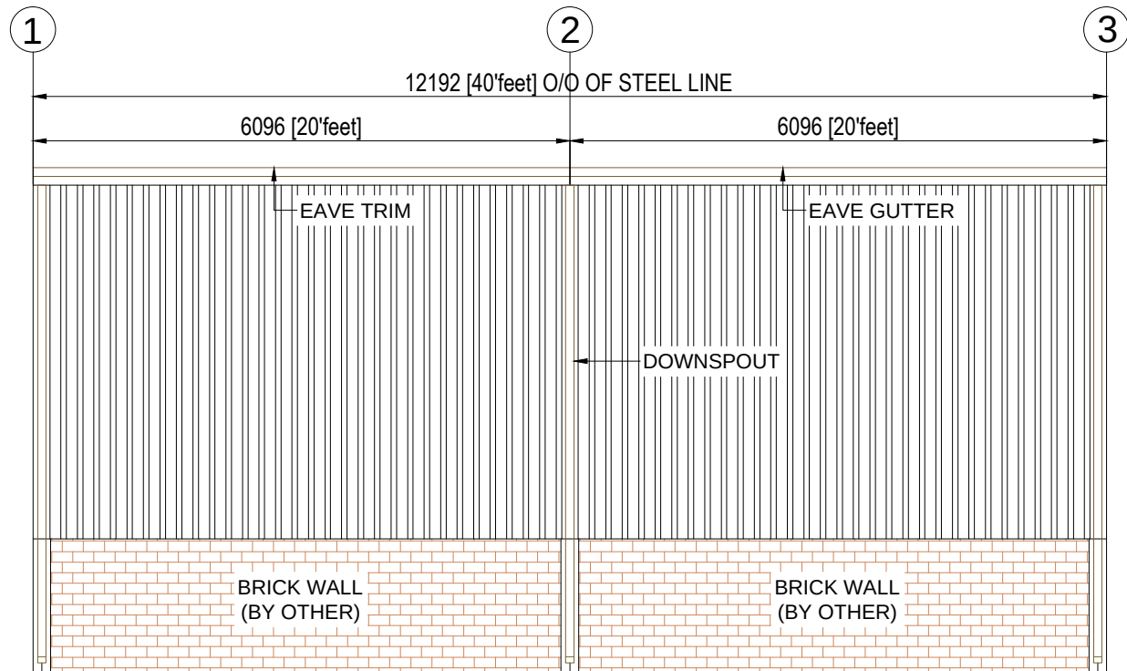
SIDE WALL SHEETING @ GRID-C
