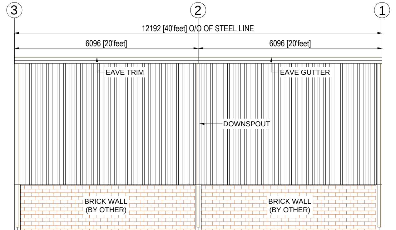
SIDE WALL SHEETING @ GRID-A
